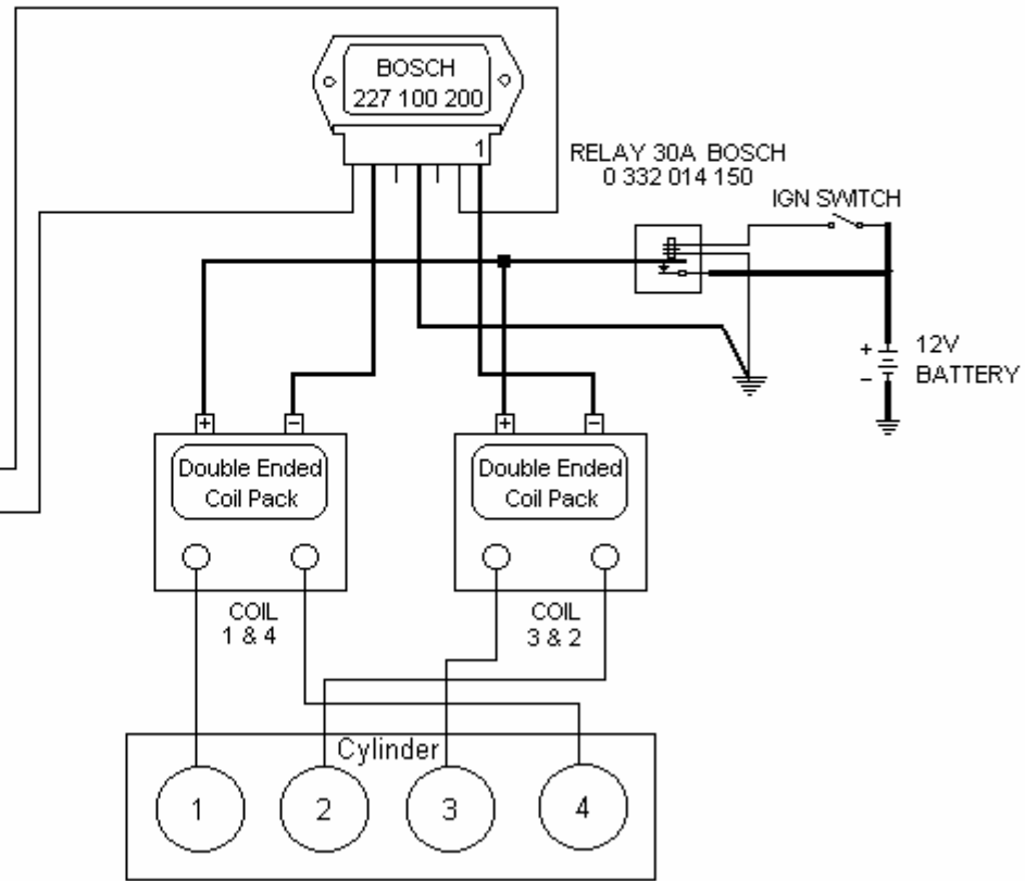
Four Cyl engine with 1,3,4,2 firing order
